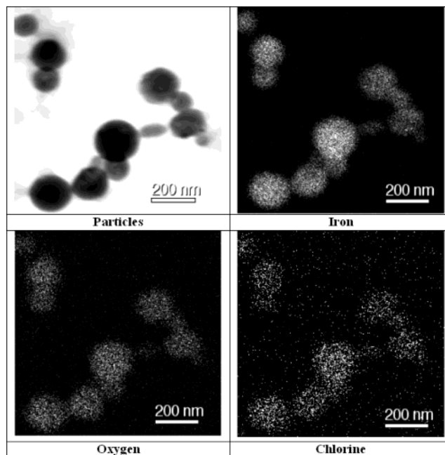
Figure 10. STEM elemental map showing the distribution of Fe, O, and Cl in the particles.
